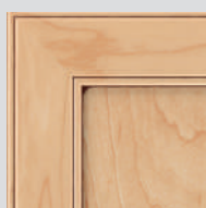
WAFER Java
